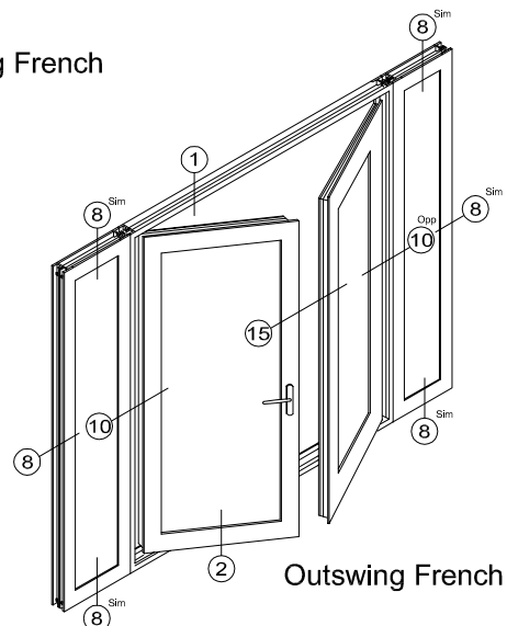
Outswing
