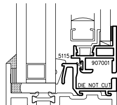
5/8" Blind/Triple Glazed
