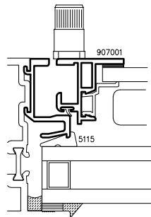
5/8" Blind/Triple Glazed
