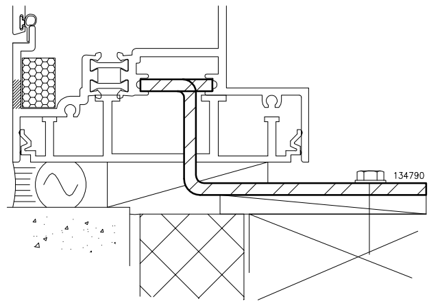
Slide-In Anchor 3/16" Formed Steel
