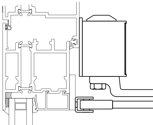
Automatic Door Closure ADA Options Available
