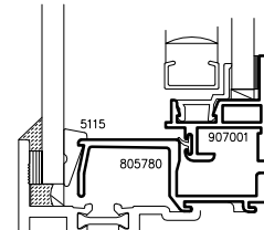
5/8" Blind/Dual Glazed
