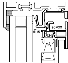
5/8" Blind/Dual Glazed
