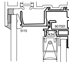
1" Blind/Dual Glazed
