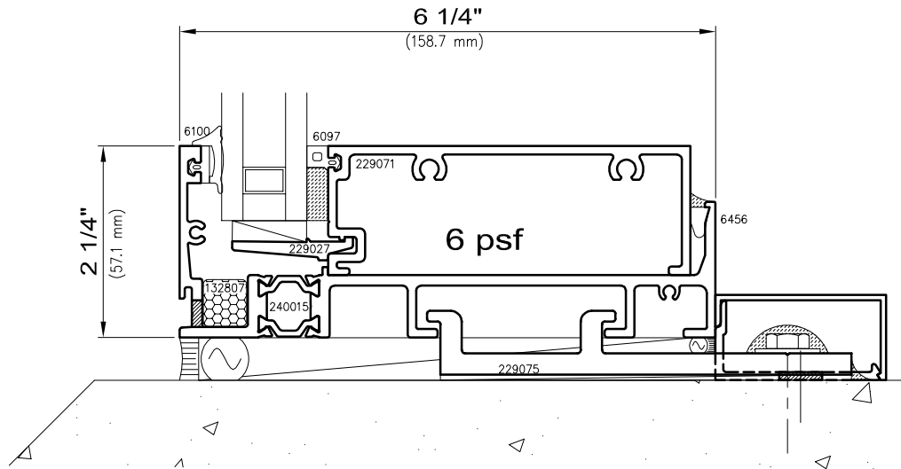
3 Vision Starter Sill - Low Profile
