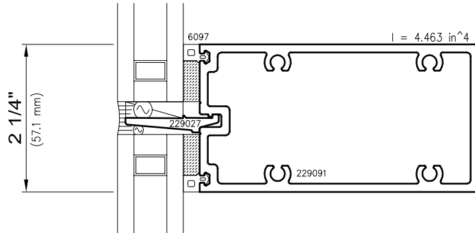
1 Vision/Vision Horizontal Intermediate
