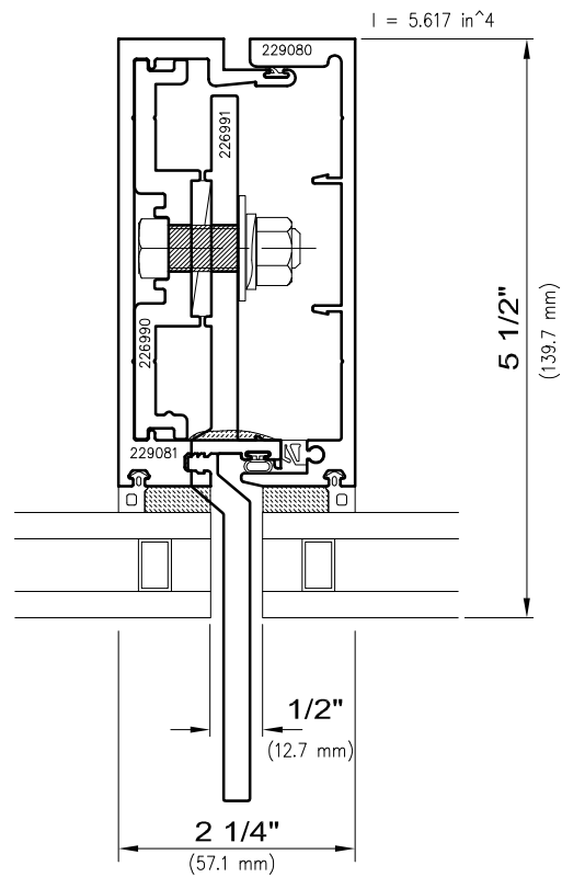
12 Vision/Vision Sunshade Bracket
