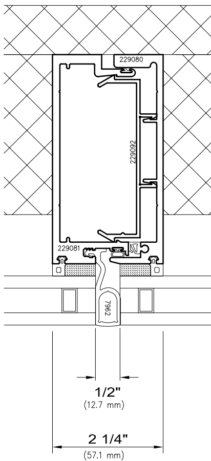
9 Spandrel/Spandrel Mullion Stack
