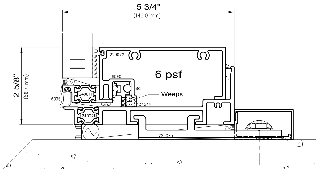
4 Vision Starter Sill - SSG
