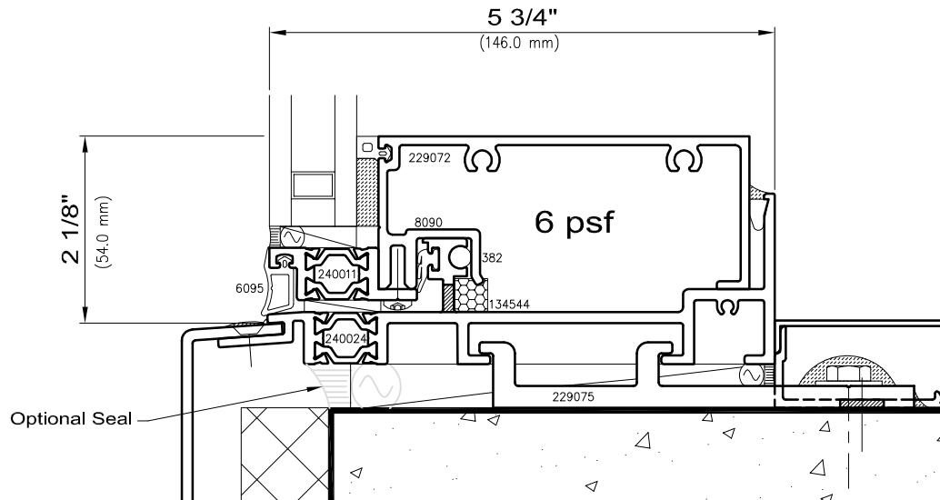
6B Vision Starter Sill - Chx. Head Slab Edge Cover
