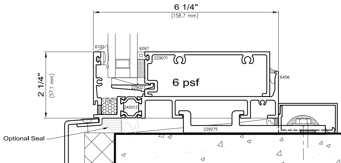
6C Vision Starter Sill - Low Profile Slab Edge Cover
