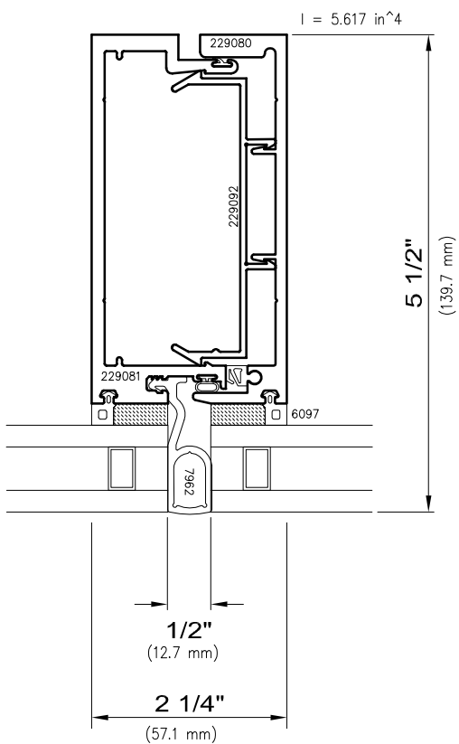
10 Vision/Vision Mullion Stack
