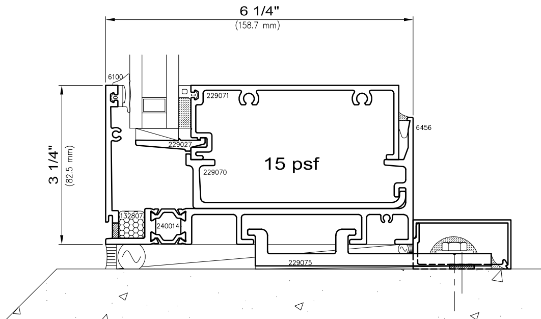
2 Vision Starter Sill - Tall Profile
