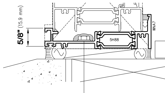
3-1/4" Sill Starter
