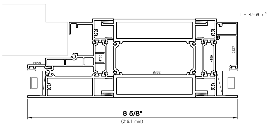
13 Operable/Fixed
