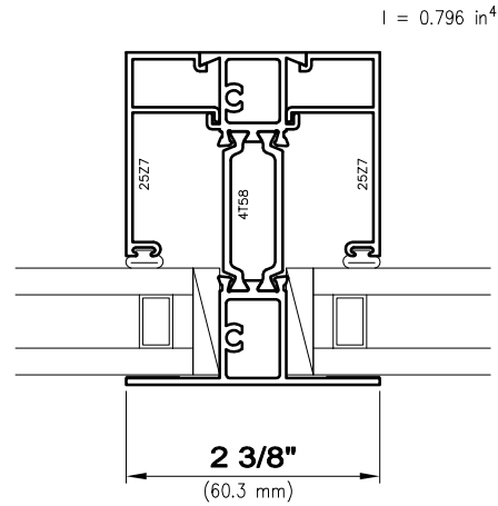
⑩A Fixed/Fixed
