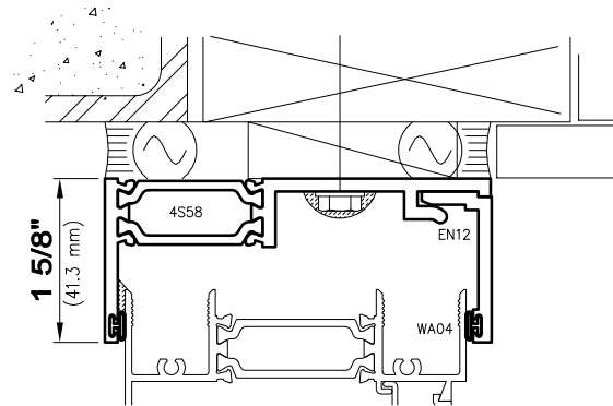
3-1/4" Head Starter
