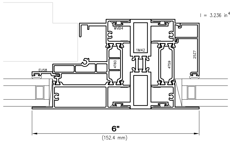
⑪ Operable/Fixed
