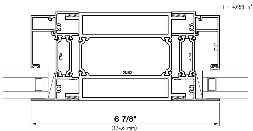
12 Fixed/Fixed
