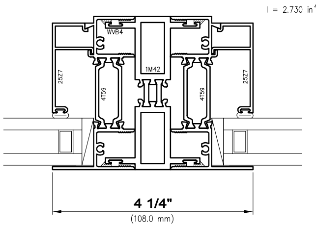
⑩ Fixed/Fixed
