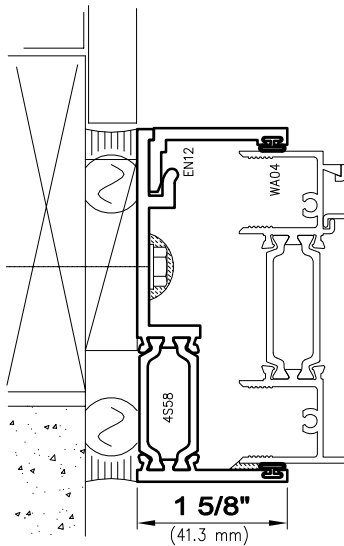
3-1/4" Jamb Starter
