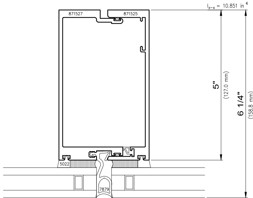
9 Vision/Vision Mullion Stack
