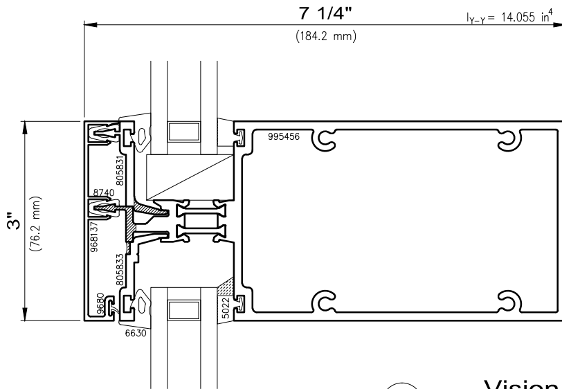
1 Vision/Vision Horizontal Intermediate
