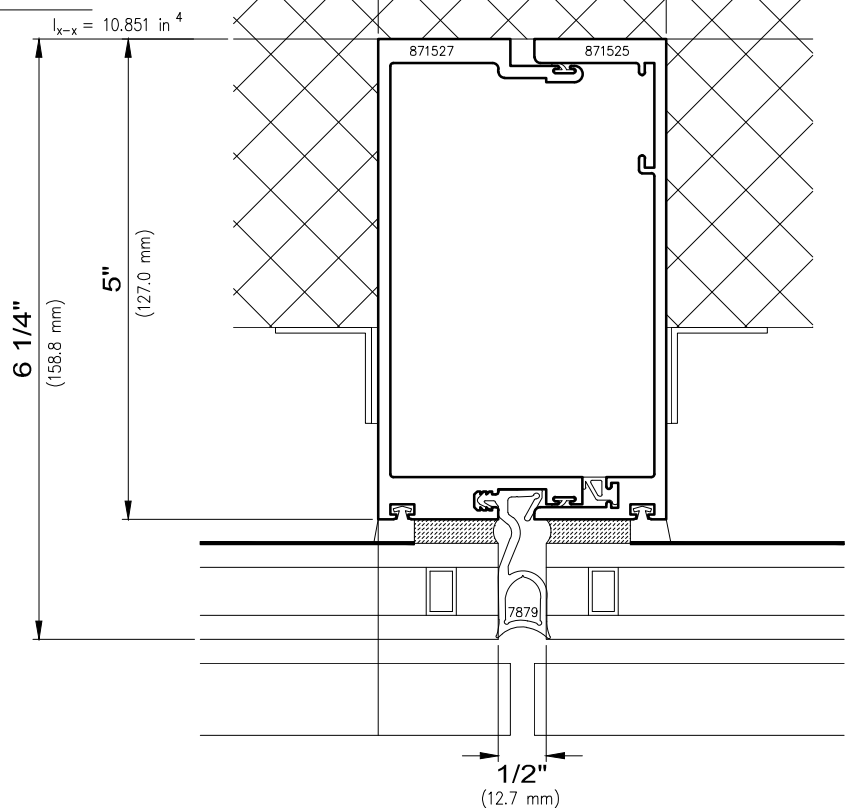
10 Spandrel/Spandrel Mullion Stack
