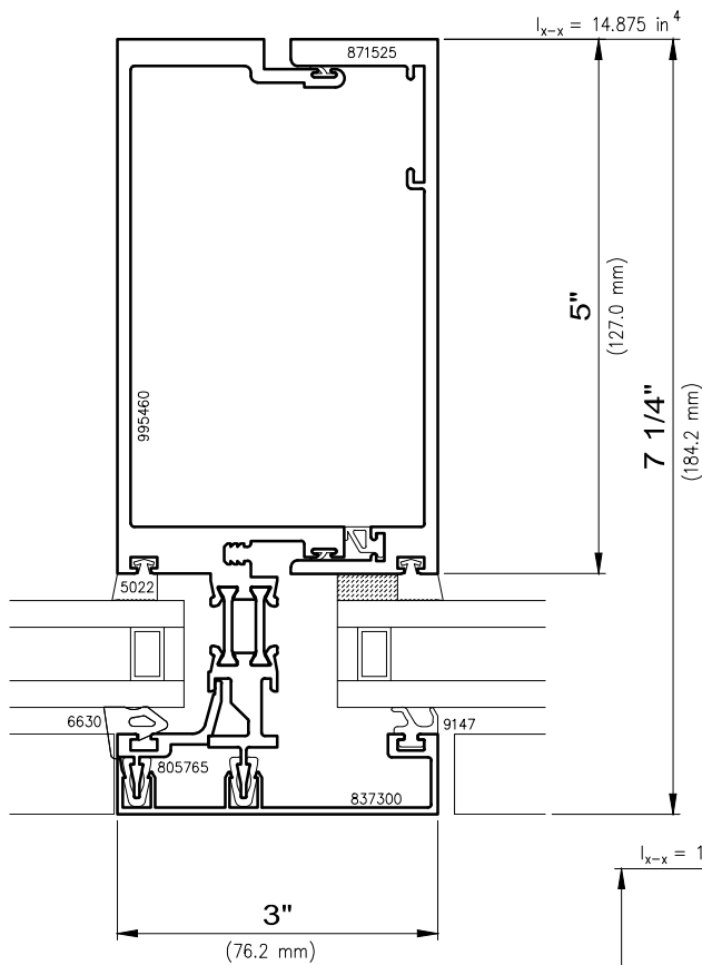
7 Vision/Vision Mullion Stack
