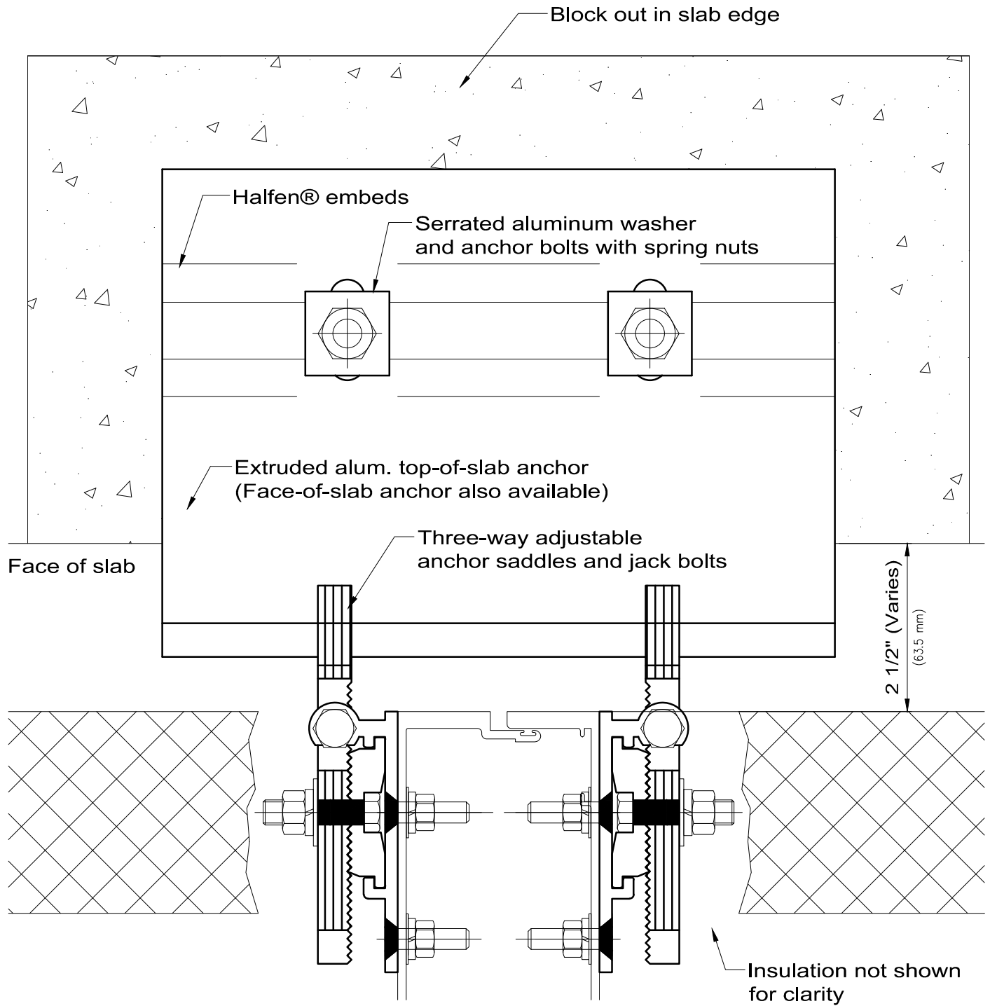
12 Plan View Unit Anchorage
