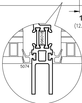
Glazing Option
