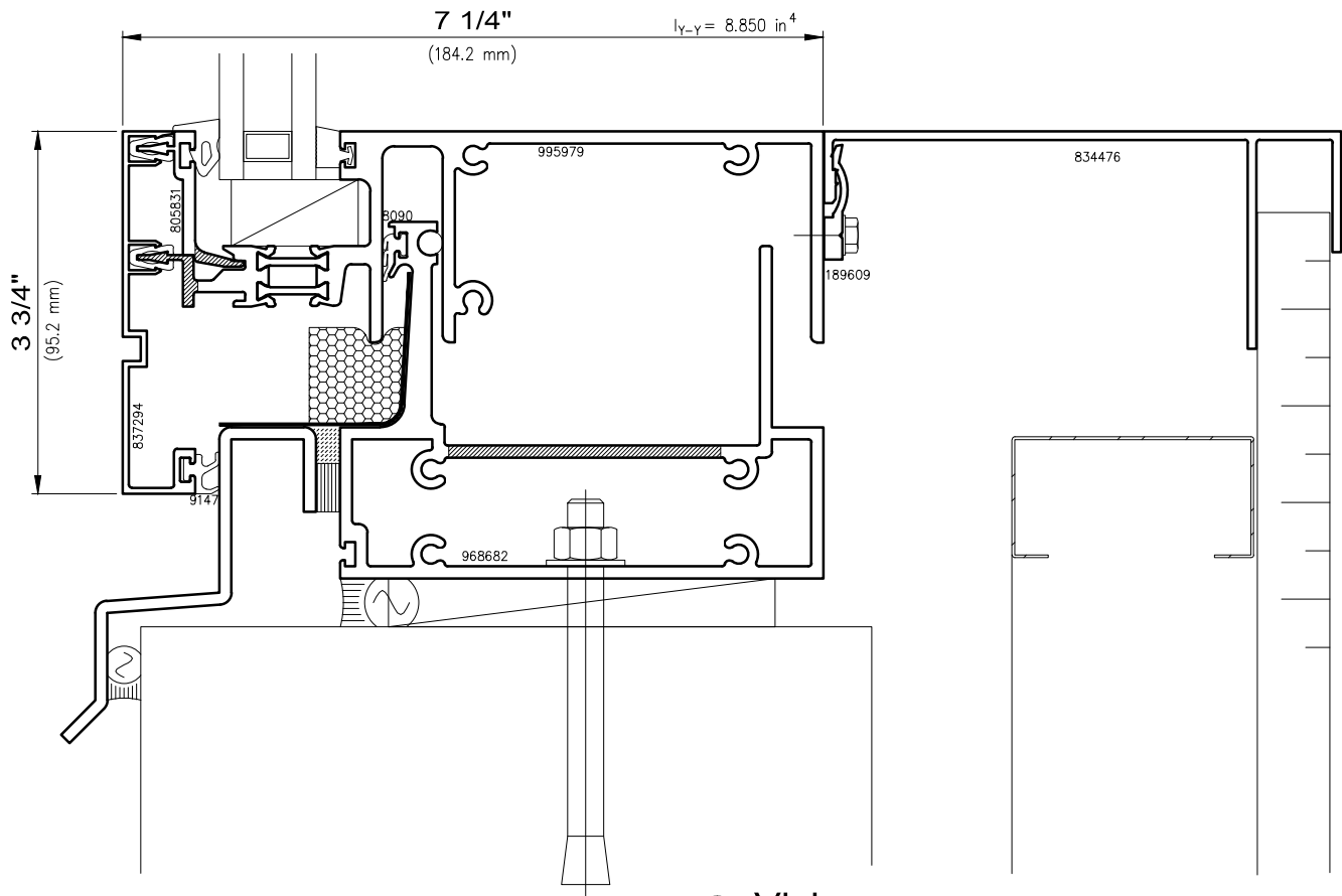
2 Vision Sill
