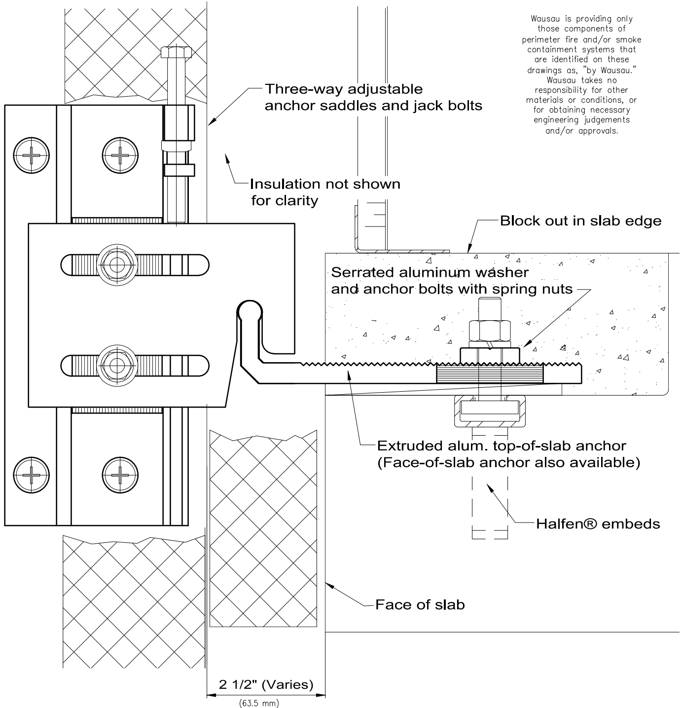
12 Section View Unit Anchorage
