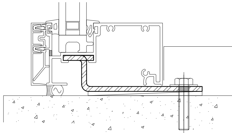
Slide-In Anchor 3/16" Formed Steel
