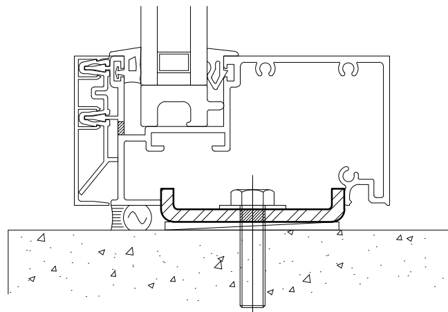
Wind-Load Anchor 3/16" Formed Steel
