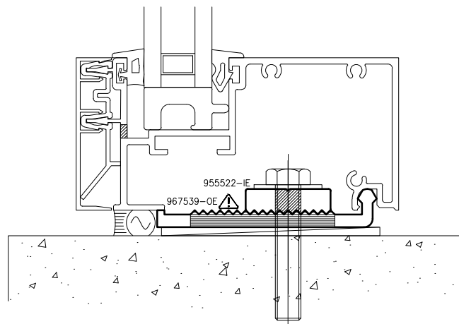
Rock-On Anchor Aluminum
