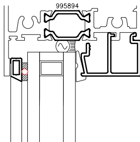
Glazed-In Muntin Grids Outside Glazed
