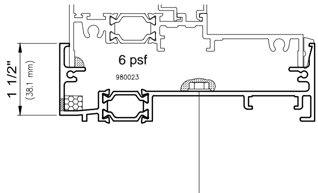
4250i-XLT 6 psf Sill Starter
