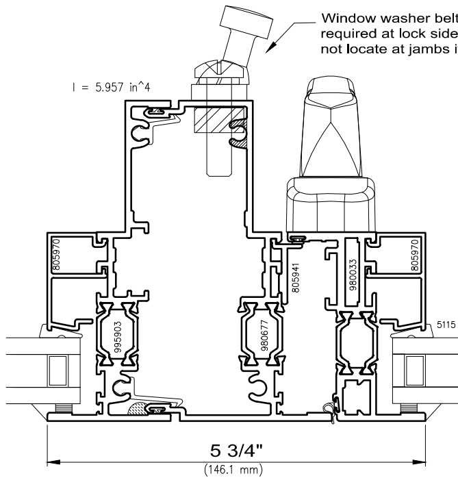
16 Fixed / Project-In Lock Side
