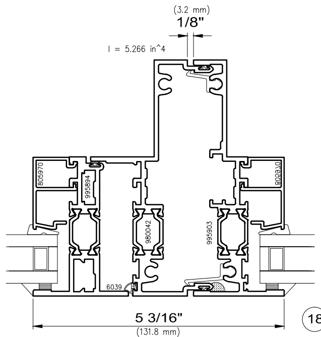
Fixed / Project-Out
