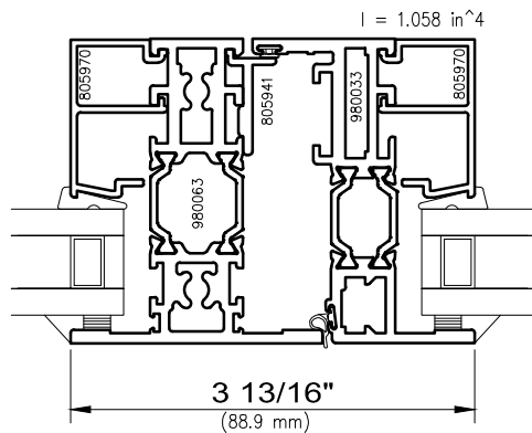
Fixed/PI Post
