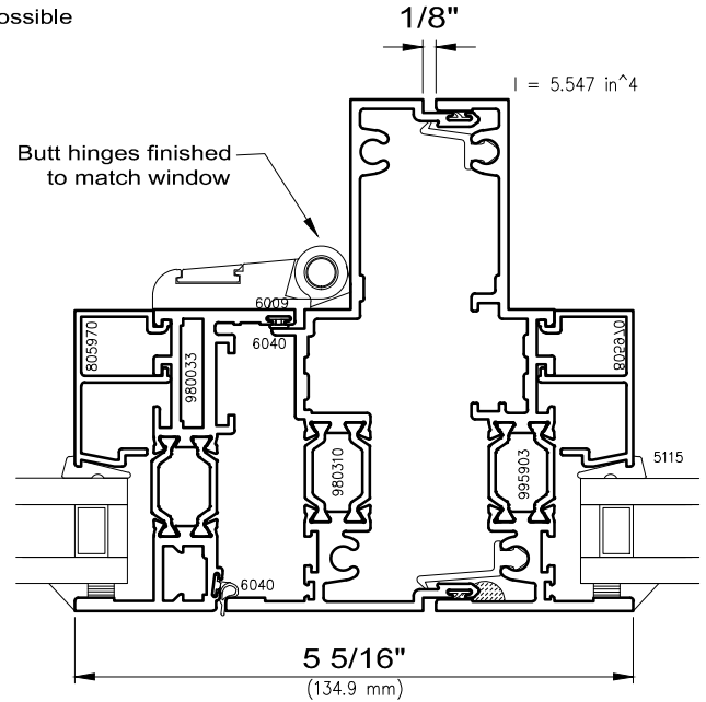
17 Fixed / Project-In Hinge Side
