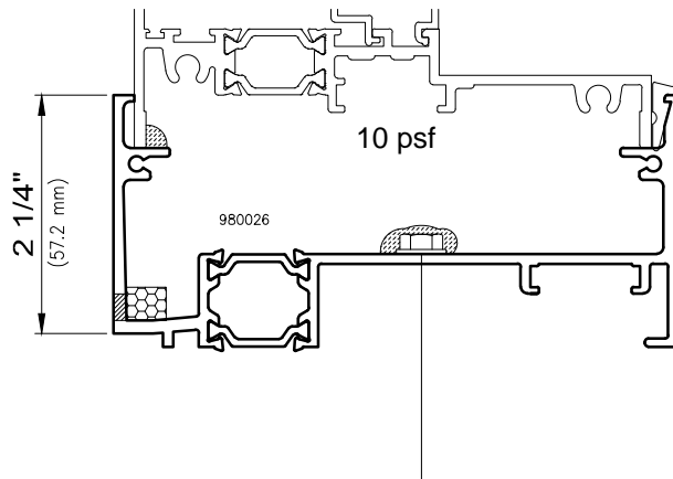
4250i-XLT 10 psf Sill Starter
