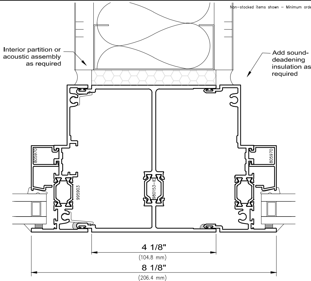
4250i-XLT H-Mullion at Partitions
