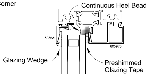
1 3/4" Triple Insulating Glass Inside Glazed
