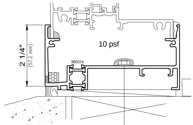
4250i Sill Starter
