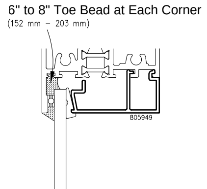
1/4" Monolithic Glass Inside Glazed
