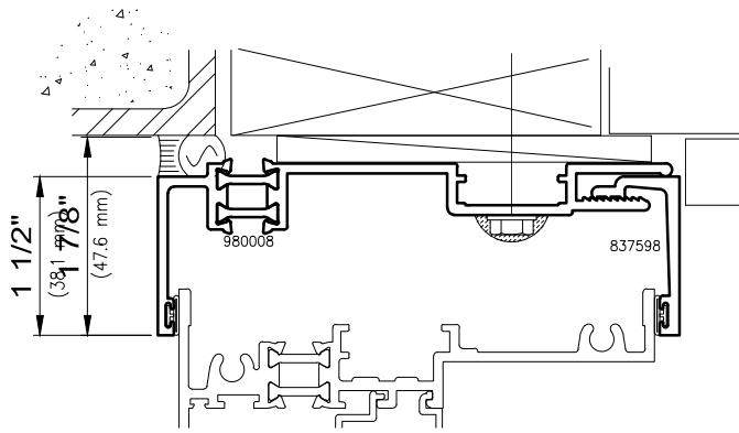
4250i Head & Jamb Starter
