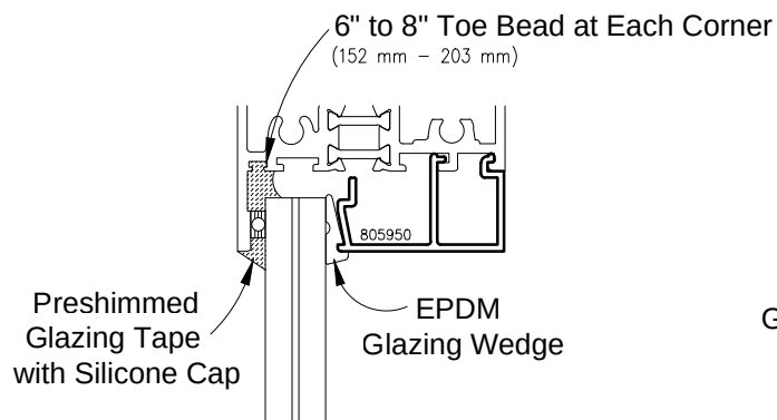
9/16" Laminated Glass Inside Glazed
