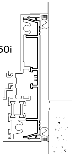
PVC Caulk Backers
