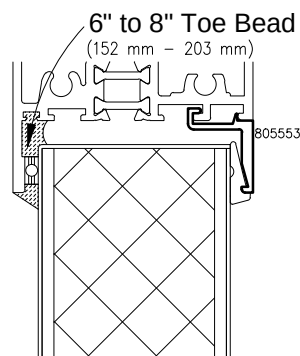
2" Panel Inside Glazed
