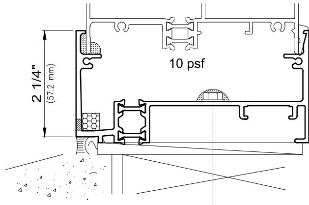
4250i Sill Starter
