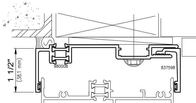
4250i Head & Jamb Starter
