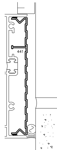
PVC Caulk Backer
