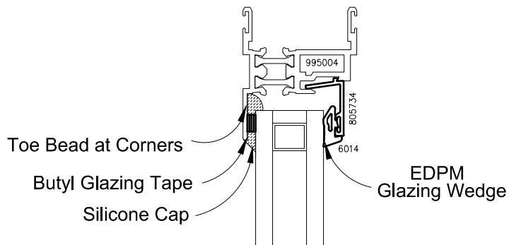
1" Insulating Glass Operable Inside Glazed
