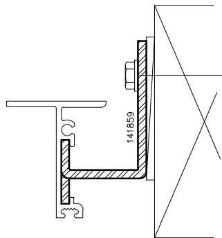
Twist-In Anchor 1/8" Formed Steel
