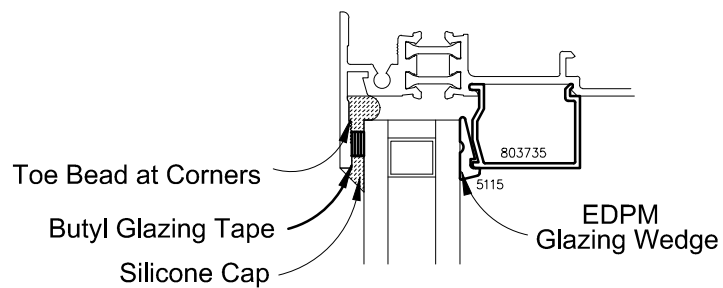
1" Insulating Glass Fixed Inside Glazed
