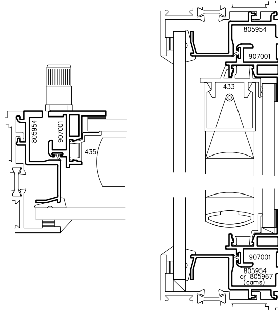
1" Blind/Dual Glazed
