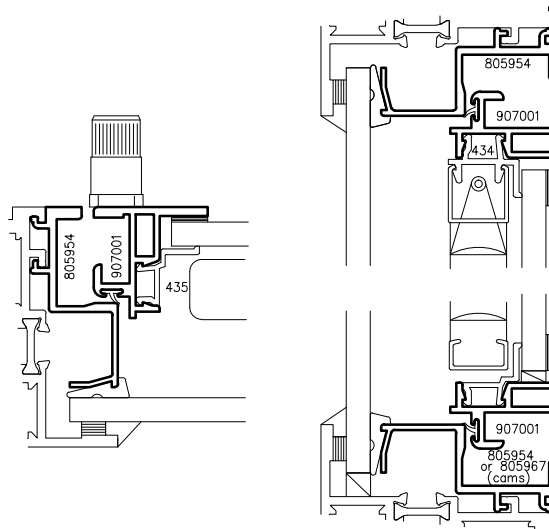
5/8" Blind/Dual Glazed
