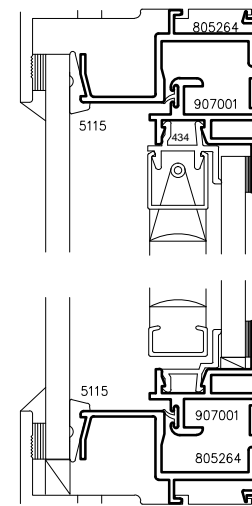
5/8" Blind/Dual Glazed
