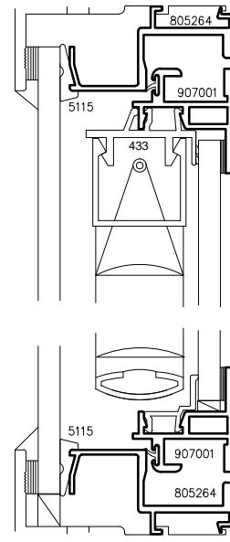
1" Blind/Dual Glazed
