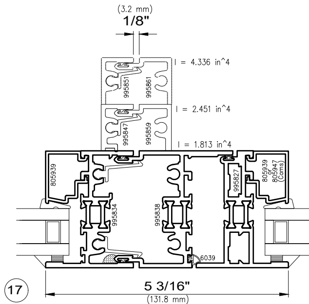
Fixed / Project-Out
