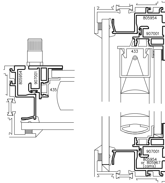
1" Blind/Dual Glazed
