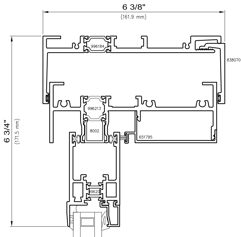
15 Operable Head Outside Slide
