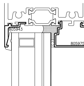
1-3/8" Spandrel Glass Outside/Inside Glazed
