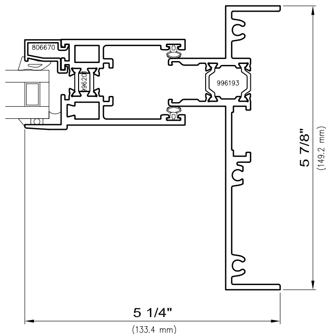
5 Operable Jamb Inside Slide
