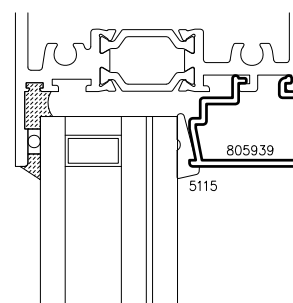
1-3/8" Insulating Glass Fixed Inside Glazed
