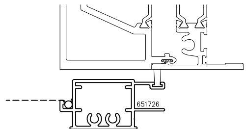
Meeting Rail
