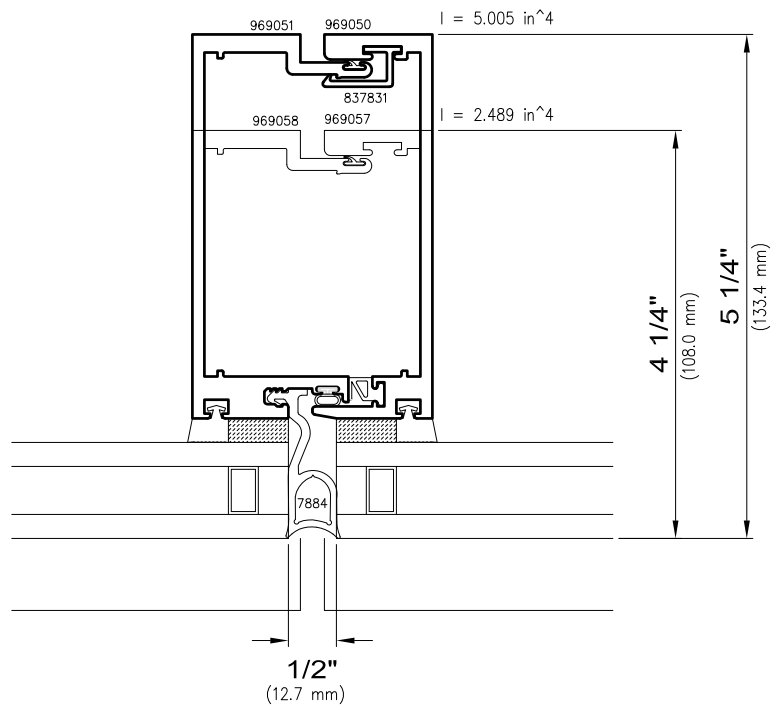
3A Vision/Vision SSG Mullion Stack
