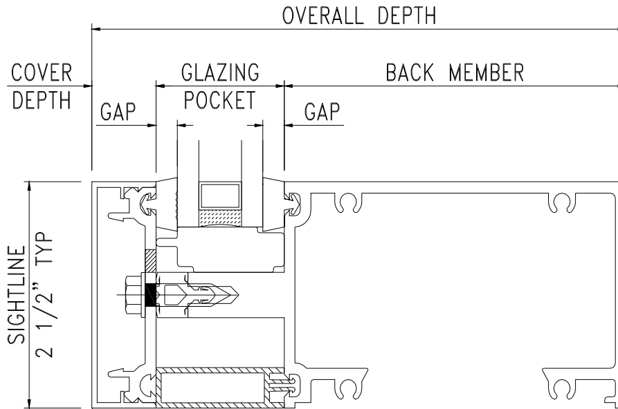
Reference Detail
