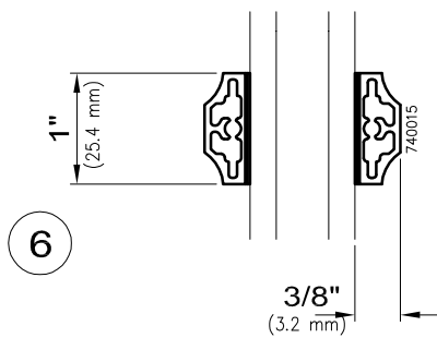
Applied Muntin Grid
