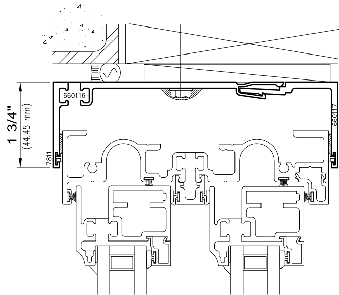
Head and Jamb Starter
